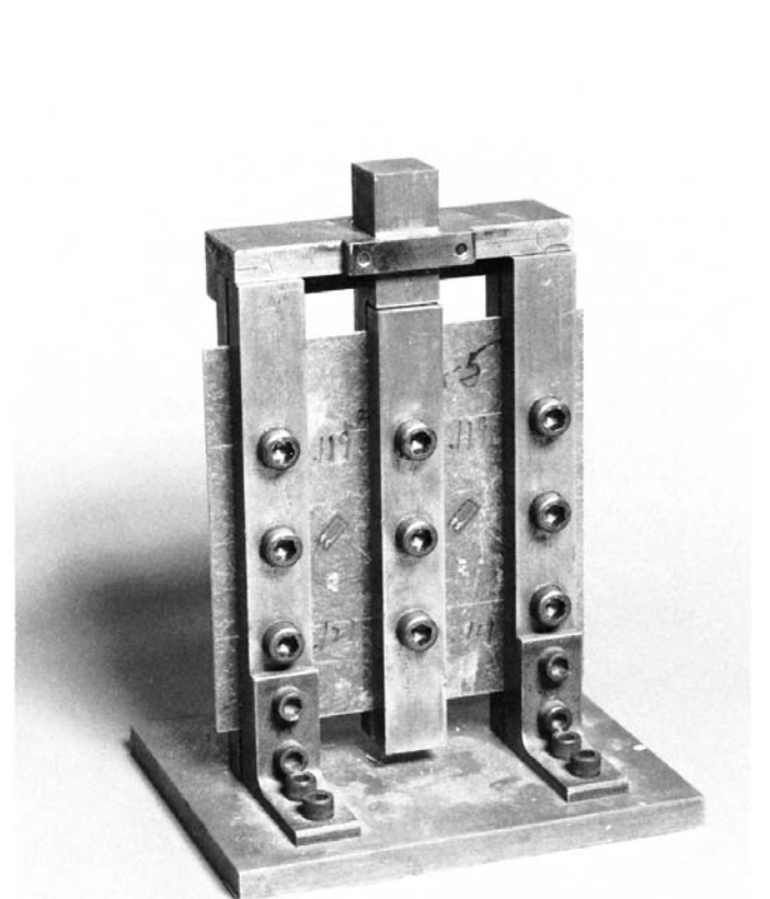
FIG. 2 Procedure A Partially Assembled Typical Test Fixture
